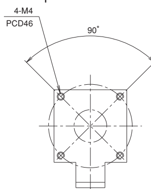
Parallel motor mounting type F□ Tension plate dimension
