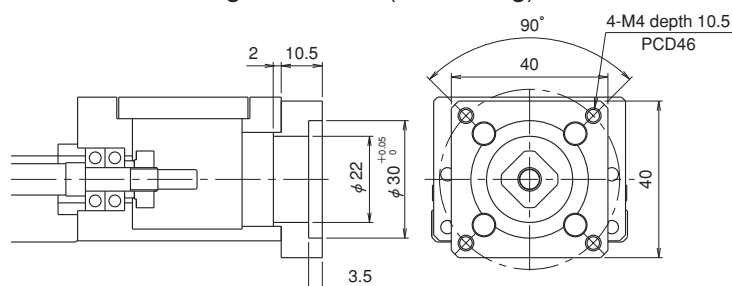
Motor bracket configuration: A1 (mass: 28g)
